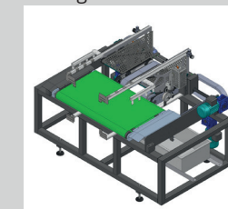
SLC continuous side sealing station
