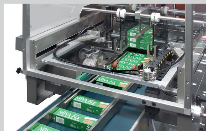
Vertical drop stacker
