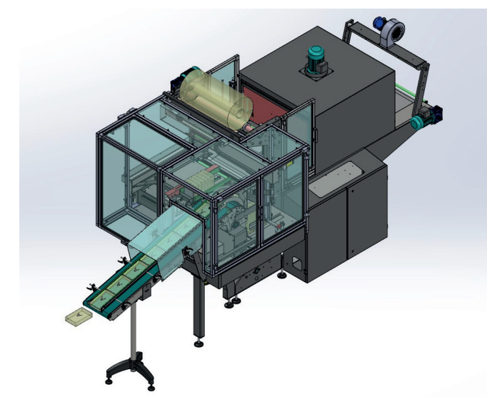
Double 90° feeding with drop stacker
