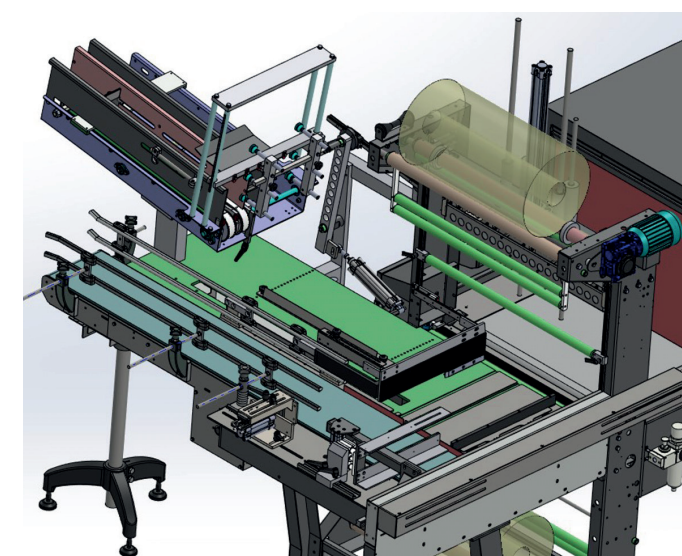
Flap insertion device (MC NEW version)
