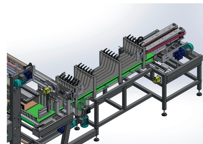
Multi-lane double 90° feeding with motorized divider
