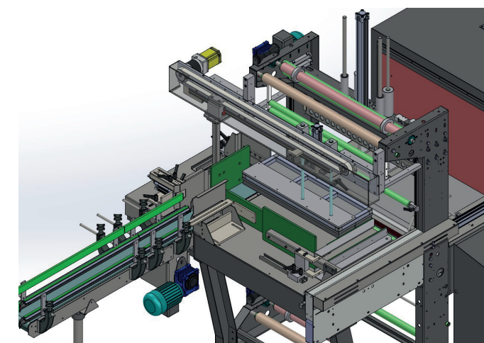
Double 90° feeding
